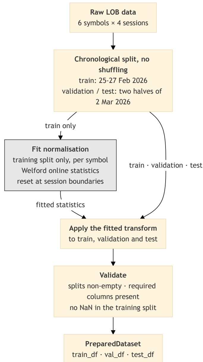
Fig. 6. Data preparation pipeline.
