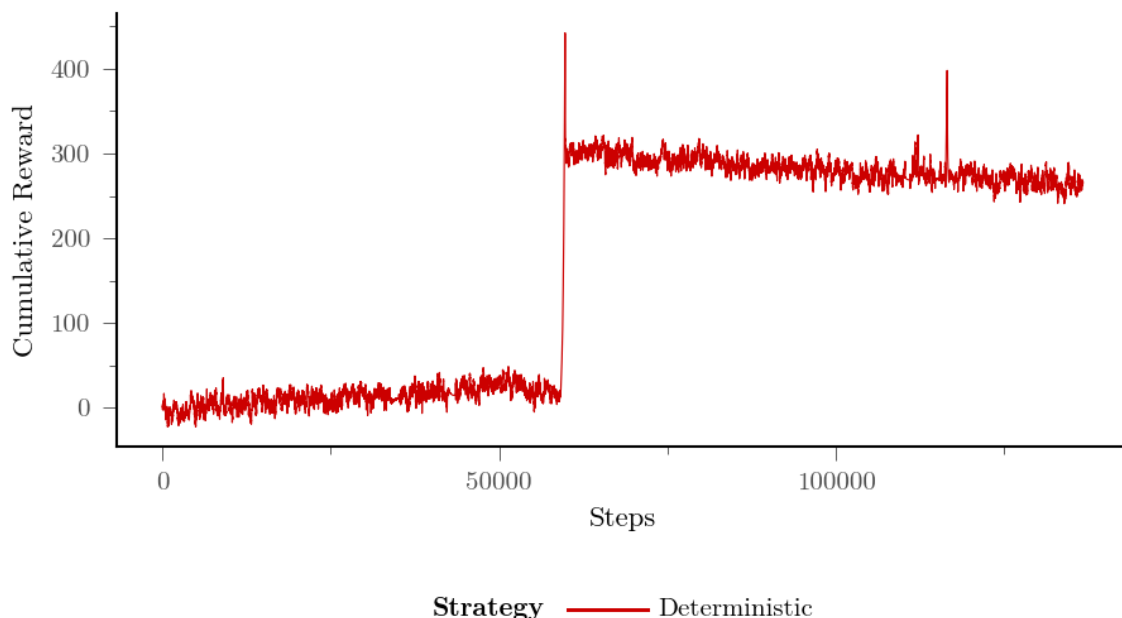
Cumulative Rewards
