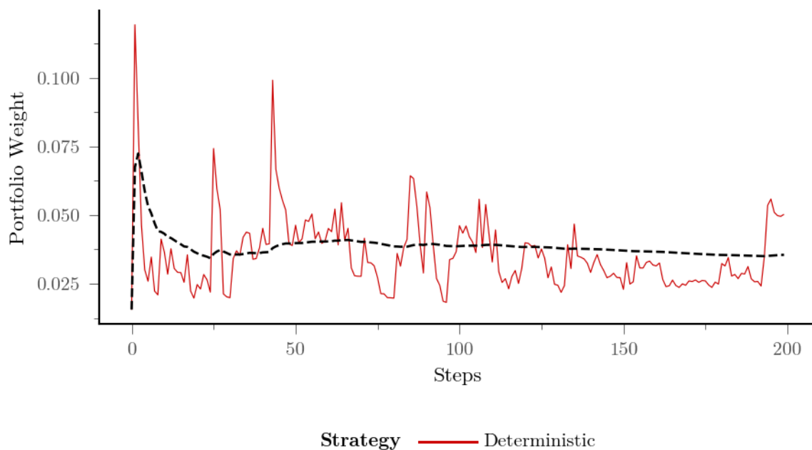
Figure 5. Portfolio allocation (position) taken by the TD3 agent at each step of the held-out evaluation rollout.
