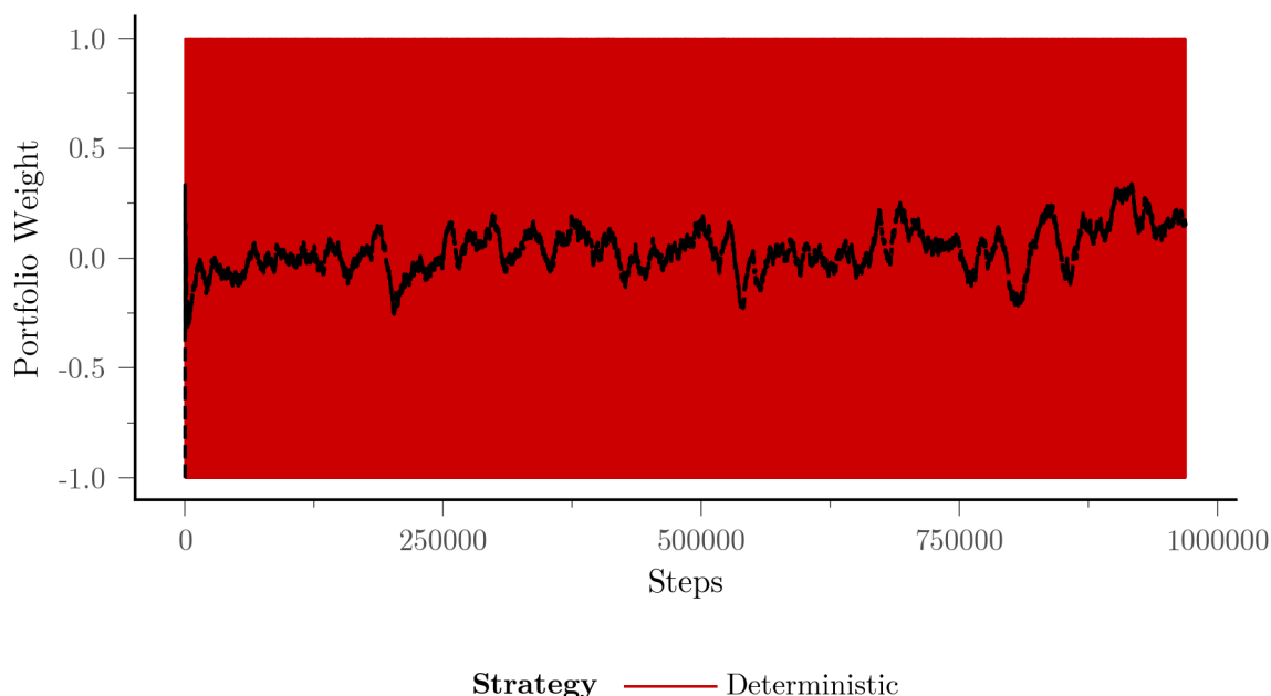
Fig. 5. Portfolio allocation (position) taken by the TD3 agent at each step of the held-out evaluation rollout. Rollout shown is AAPL from the same 3,000,000-step checkpoint as the results tables, evaluated over 969,218 test-split steps (run d7c200923b).
