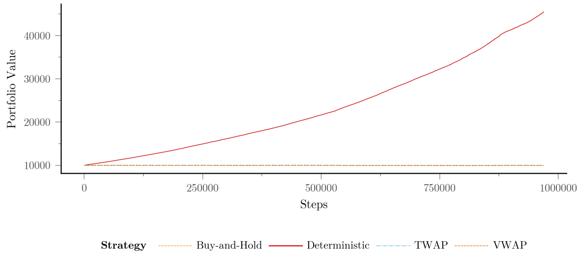
Fig. 3. Portfolio value over the held-out evaluation window for the TD3 agent and benchmark strategies. Rollout shown is AAPL from the same 3,000,000-step checkpoint as the results tables, evaluated over 969,218 test-split steps (run d7c200923b).
