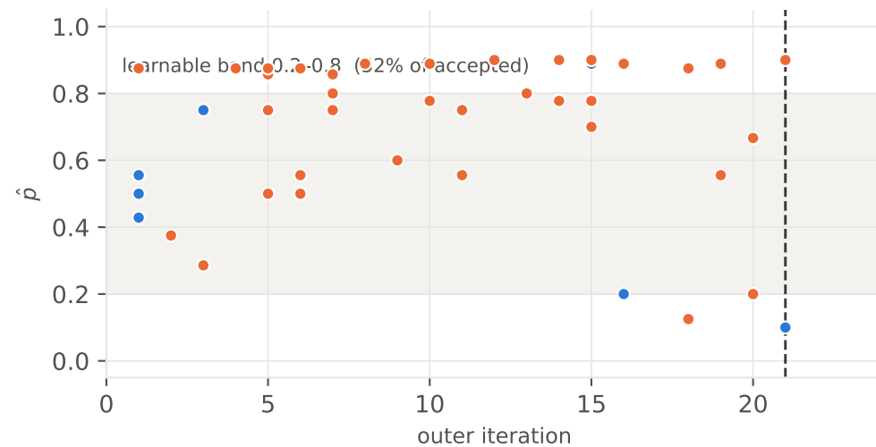
C · Solver pass rate \hat{p} of accepted children at insertion
