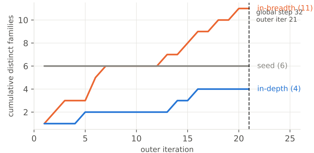
B · Distinct problem families first observed, by origin
