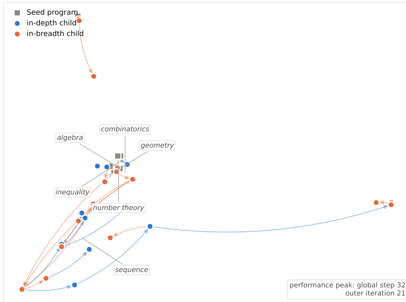
A · Problem space (SVD of TF-IDF problem text), all archived programs
