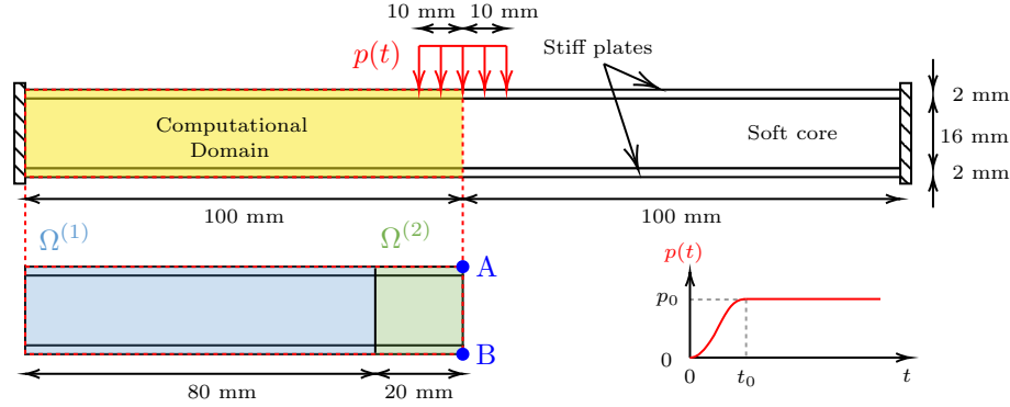
Fig. 21 Impact of a sandwich plate. Material properties of stiff plates: mass density \rho = 27 \times 10^{-10} ton/mm 3 , Poisson's ratio \nu = 0.3 , and elastic modulus E = 70,000 MPa. Material properties of the soft core: mass density \rho = 9 \times 10^{-10} ton/mm 3 , Poisson's ratio \nu = 0.3 , and elastic modulus E = 7,780 MPa. A smooth step function with t_0 = 10^{-5} sec and p_0 = 1 MPa is used to mimic the impact load p(t) .
