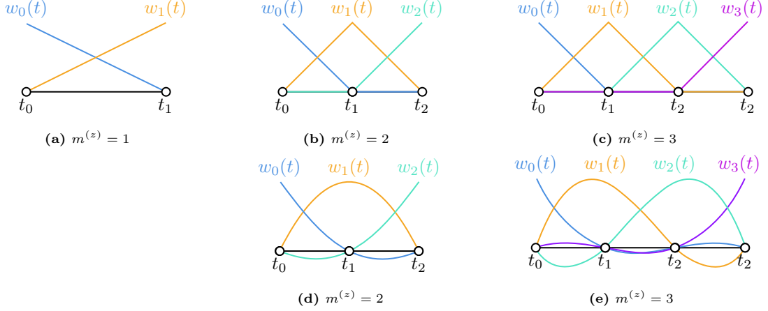
Fig. 5 Examples of weight functions used for interpolation: (a), (b), (c) piecewise-linear interpolation; and (a), (d), (e) Lagrange polynomial.
