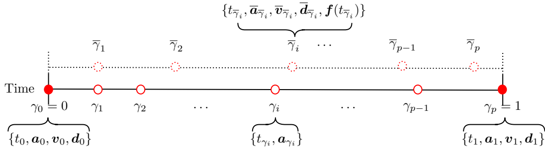
Fig. 2 Representation of p -stage GRKN scheme.
