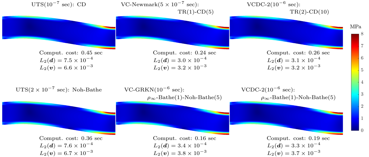
Fig. 23 Snapshots of von Mises stress and deformation (deformation scaling factor is 500) at time t = 6 \times 10^{-5} \text{ sec} for the impact problem.
