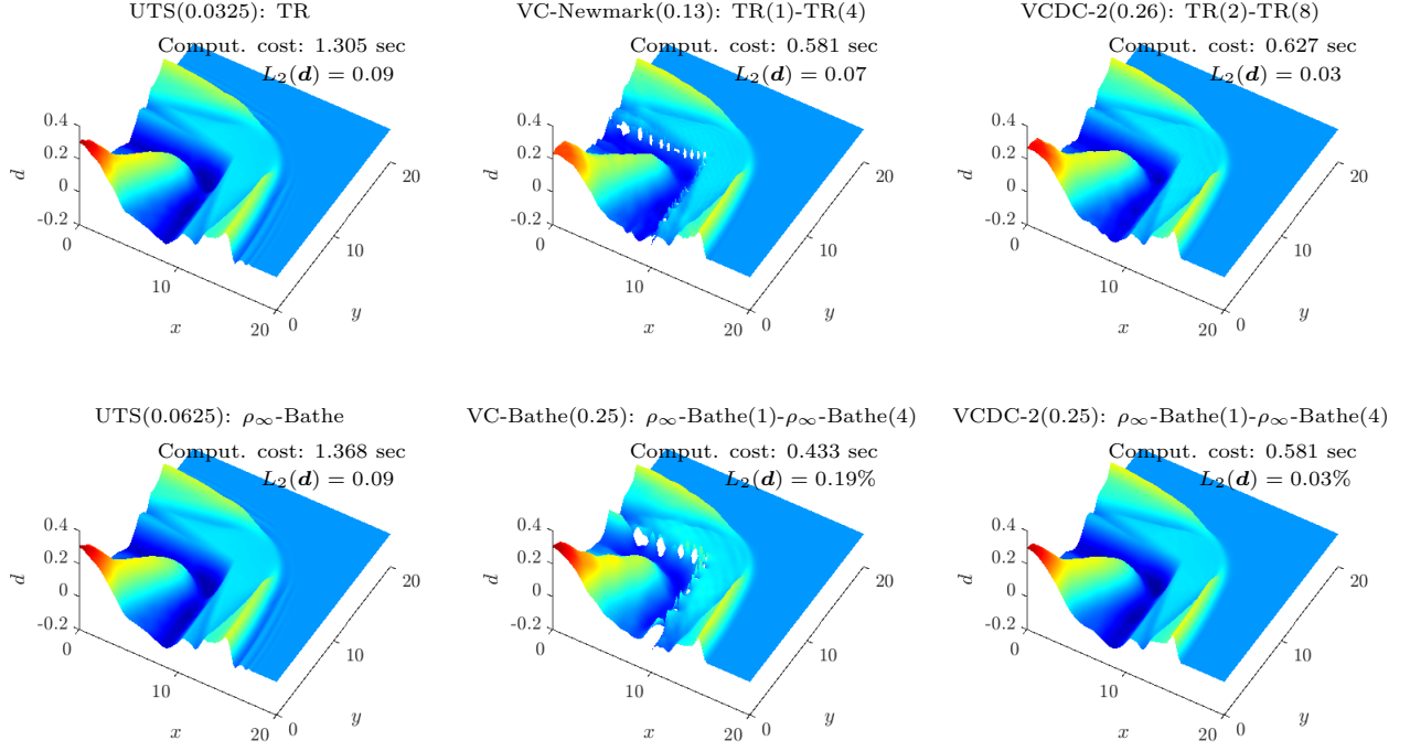
Fig. 14 Snapshots of displacement at time t = 8 for the scalar wave propagation problem when h = 0.2 .
