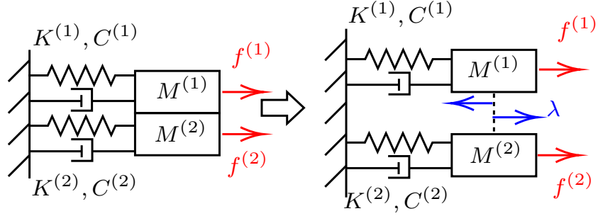
Fig. 7 Split single-degree-of-freedom (SDOF) problem with two subdomains
