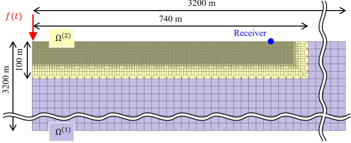
Fig. 18 Spatial mesh discretization for the 2D Lamb's problem with two subdomains. In subdomains \Omega^{(1)} and \Omega^{(2)} , the characteristic lengths are h^{(1)} = 20 m and h^{(2)} = 2 m, respectively.
