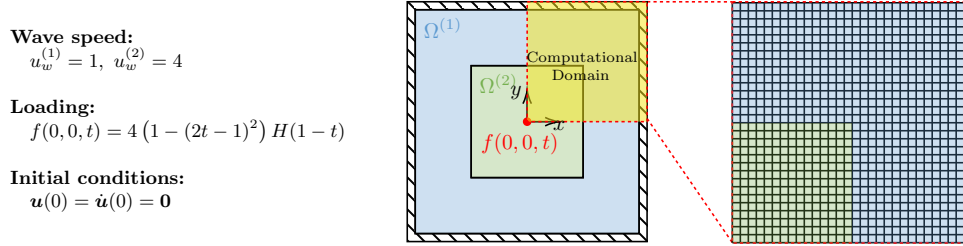
Fig. 13 Pre-stressed membrane with two different media
