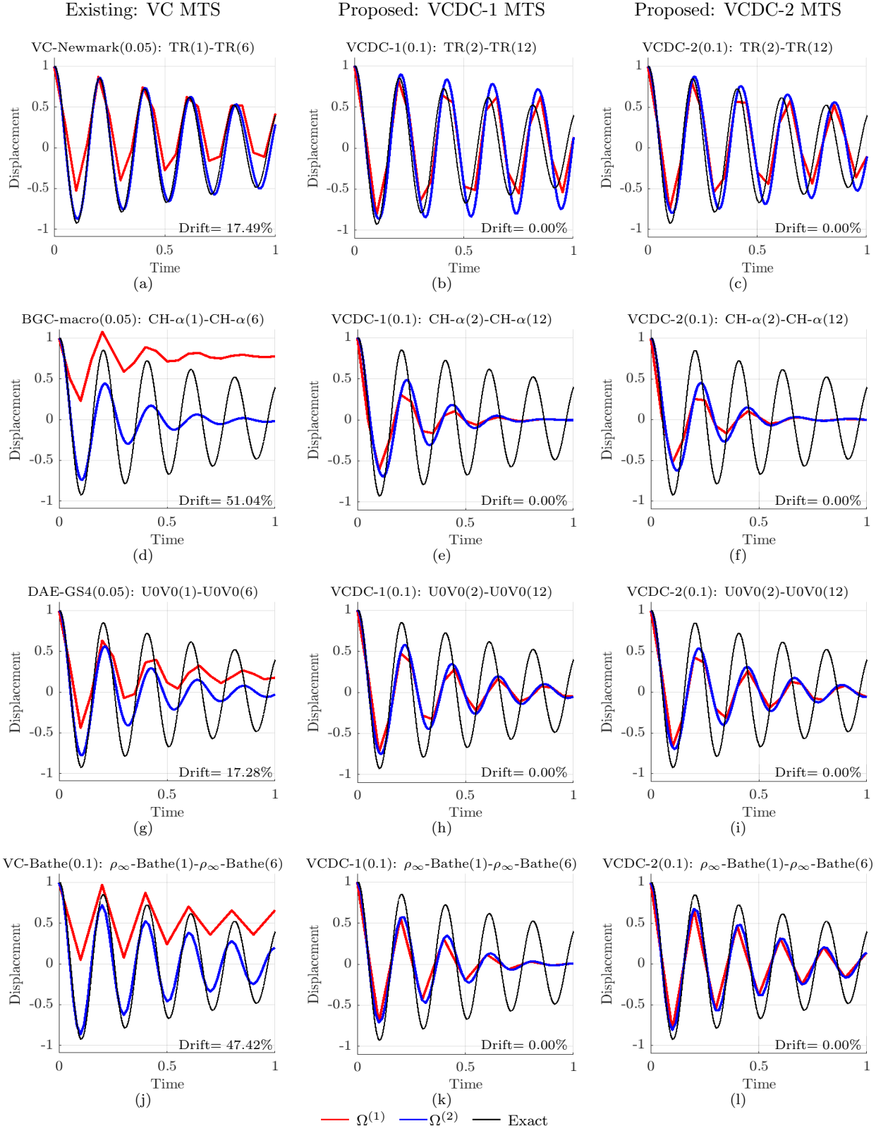
Fig. 8 Comparison of drifts in displacement for the split-SDOF problem obtained using different existing and proposed MTS methods. Different MTS methods are denoted as (MTS name )( \Delta T ): GRKN( m^{(1)} )-GRKN( m^{(2)} ).
