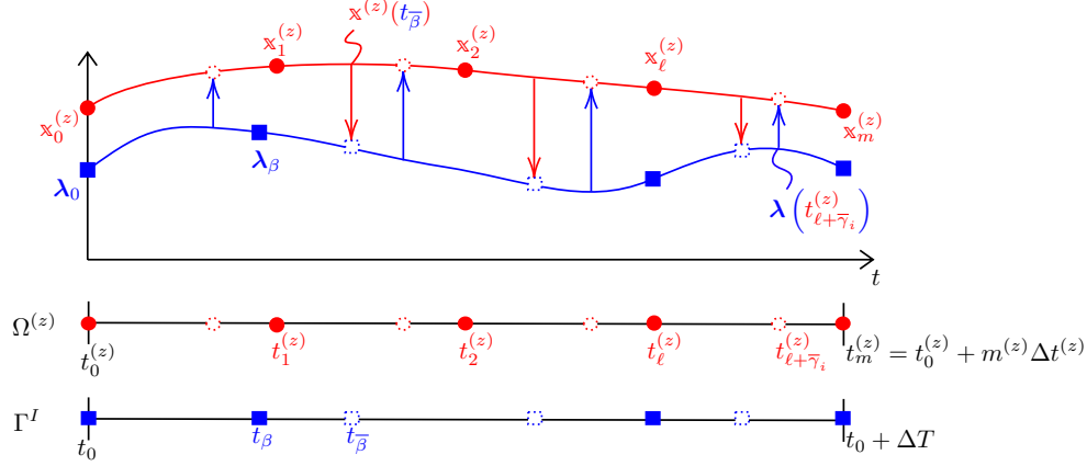
Fig. 4 Multi-time-step trajectories of subdomain state vectors \mathbf{x}^{(z)}(t) and Lagrange multipliers \boldsymbol{\lambda}(t) . Note that the subdomain state vectors \mathbf{x}_\ell^{(z)} are only computed at \Delta t^{(z)} intervals and Lagrange multipliers \boldsymbol{\lambda}_\beta are only computed at times t_\beta . The exchange of information between subdomain \Omega^{(z)} and the interface \Gamma^I at all other times t , is facilitated by interpolating these quantities with user-defined functions.
