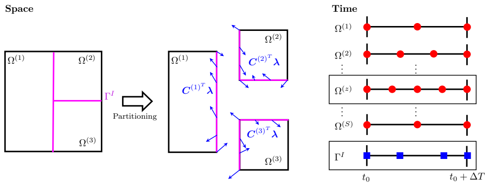
Fig. 3 Spatial domain decomposition of a problem into multiple subdomains that are integrated using different GRKN schemes and different time steps. A single block time step \Delta T is used to advance the coupled system of subdomains.
