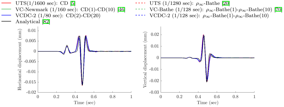
Fig. 19 Time history of horizontal and vertical displacements at (x, y) = (640, 3200) m for the 2D Lamb's problem.
