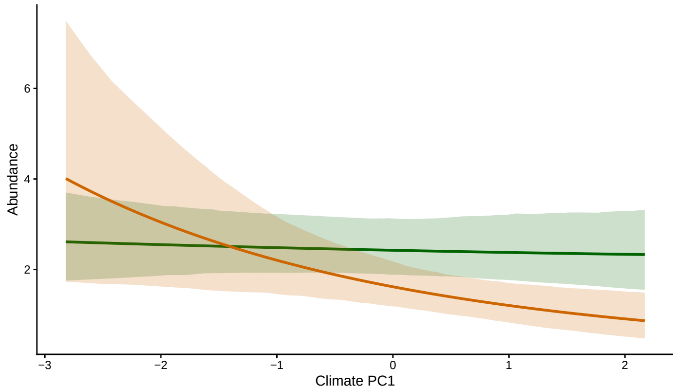
Lynx abundance vs PC1 at low/high HF
