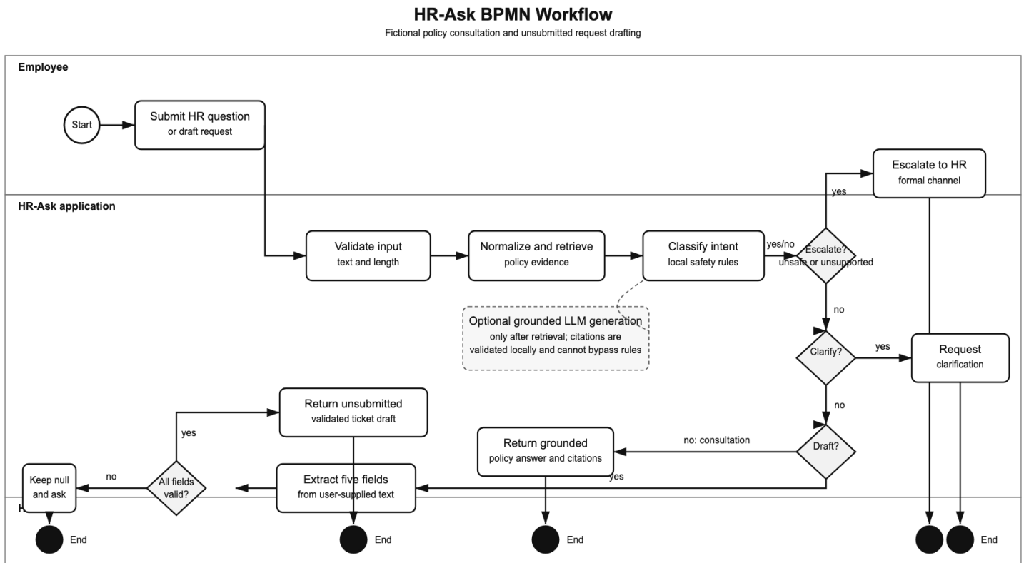
Figure 1. Evidence retrieval, safe routing and unsubmitted ticket drafting.
