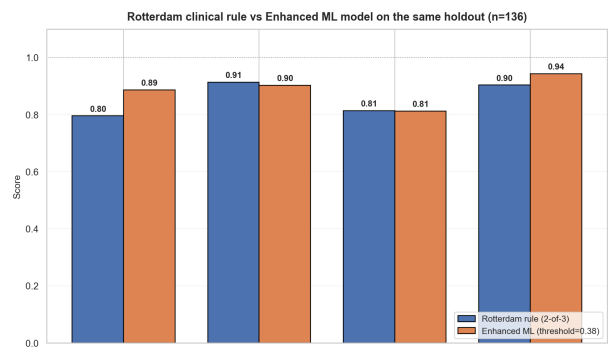
Figure 16. Rotterdam rule vs enhanced ML, side-by-side metrics.
