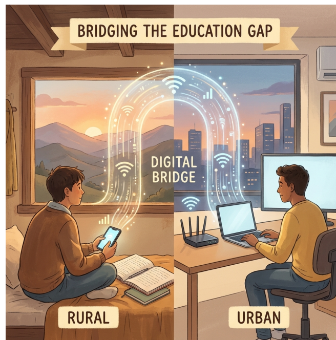
Figure 7.1: Education Revolution
