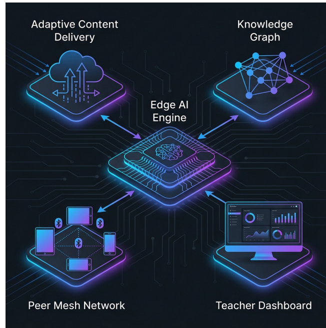
Figure 8.1: EduBridge Architecture
