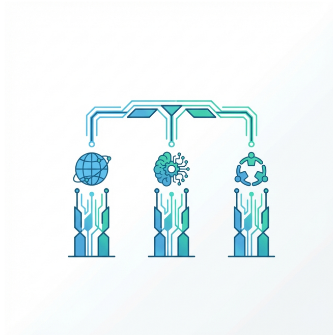
Figure 6.1: Concept Diagram
