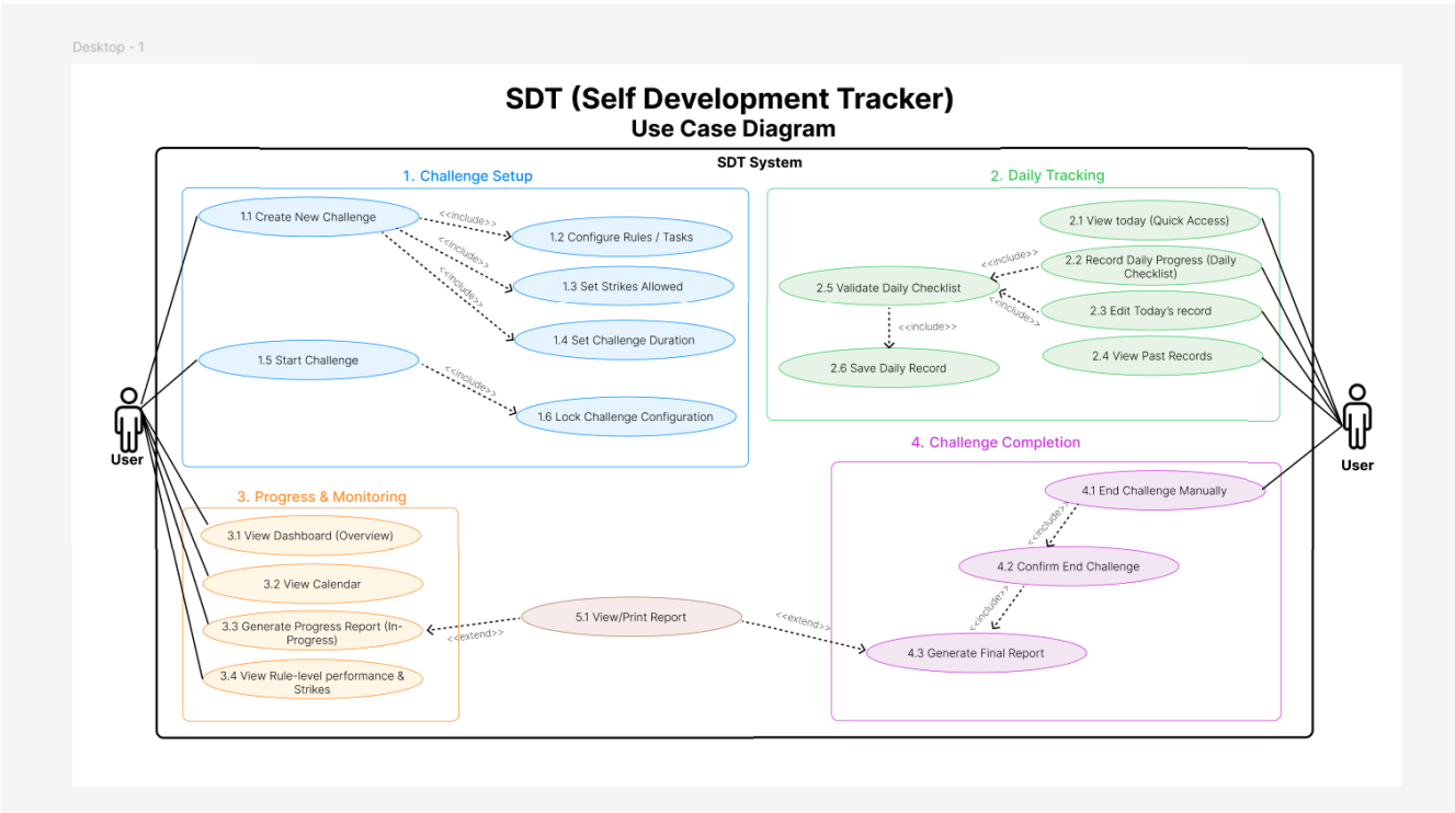
Figure 1. SDT V1 Use Case Diagram
