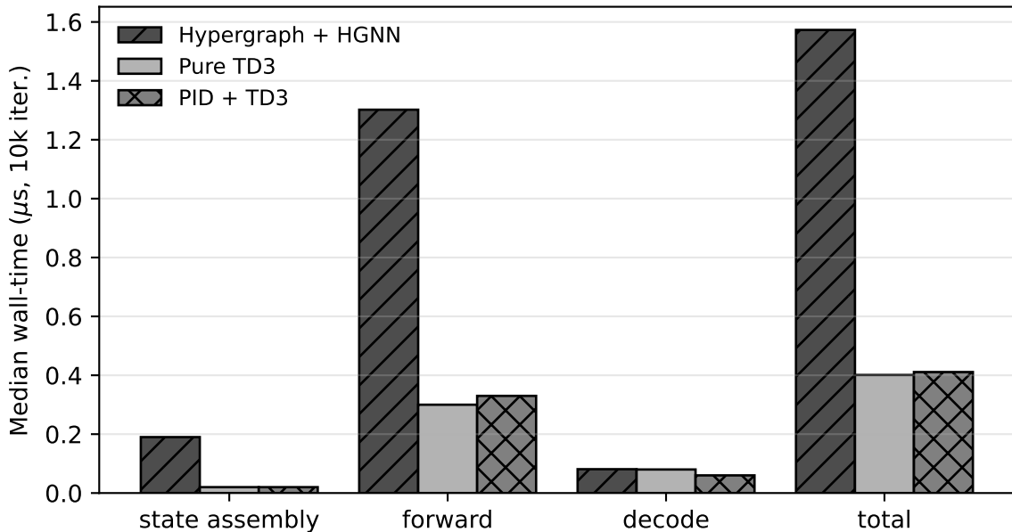
Exp. 3 control-cycle timing, canonical grasping scenario
