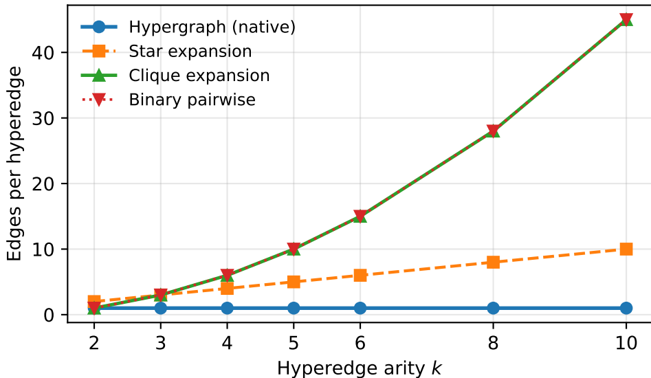
Representational cost per hyperedge vs. arity
