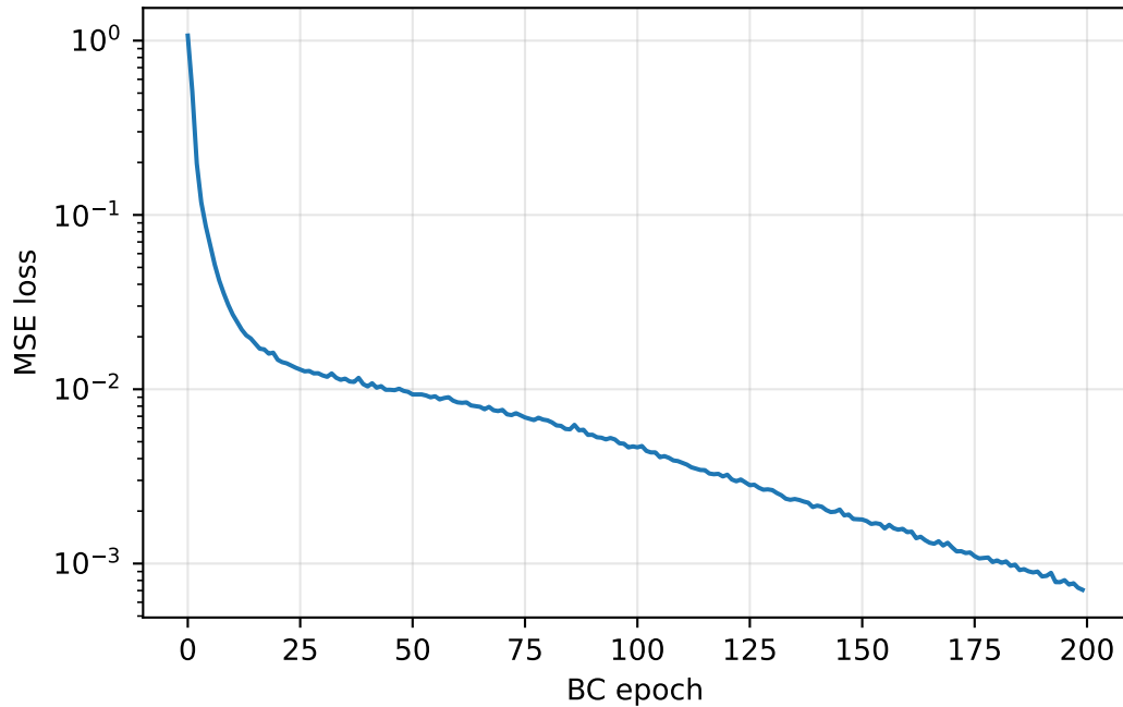
Behaviour-cloning loss
