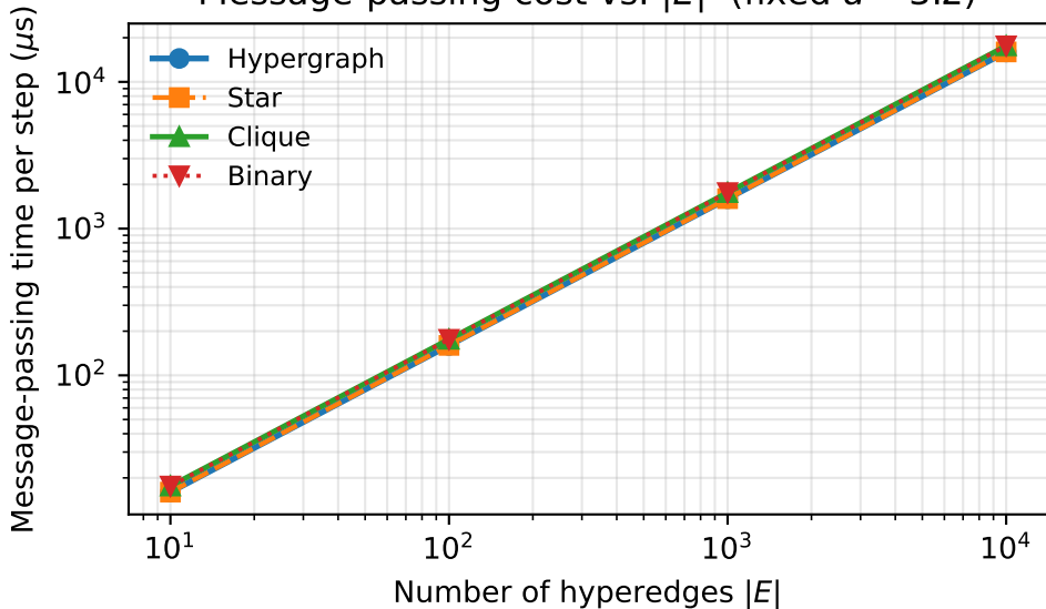
Message-passing cost vs. |E| (fixed \bar{d} = 3.2 )
