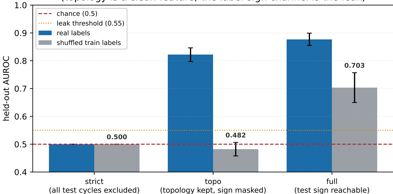
Cycle/HSiKAN method: leakage appears only at R_{\text{full}} (topology is a clean feature; the label-sign channel is the leak)
