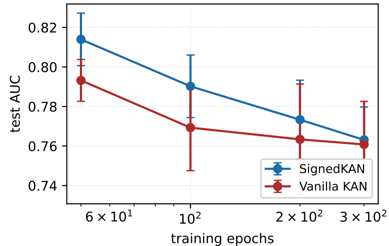
Bitcoin Alpha
