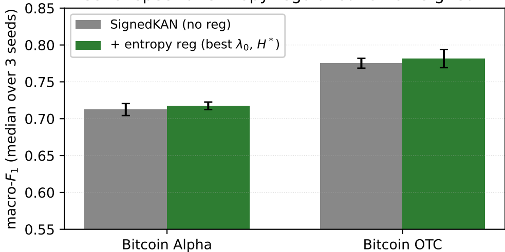
Effect of spectral-entropy regularisation on SignedKAN
