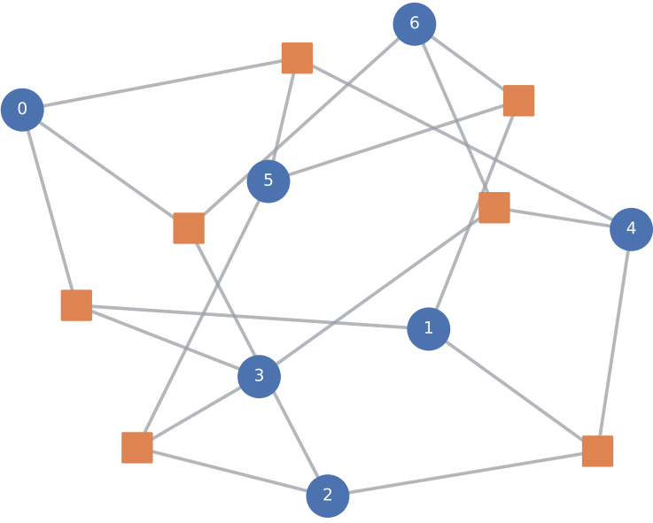
Fano S(2,3,7) = PG(2,2) projective, 7 points 7 lines
