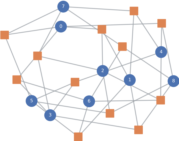
Steiner S(2,3,9) = AG(2,3) affine, 9 points 12 lines
