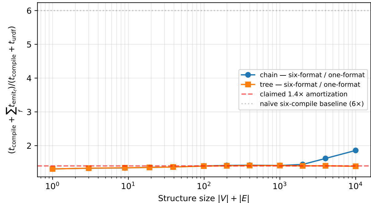
Amortization witnessing projection-emission commutativity (Prop. 3)
