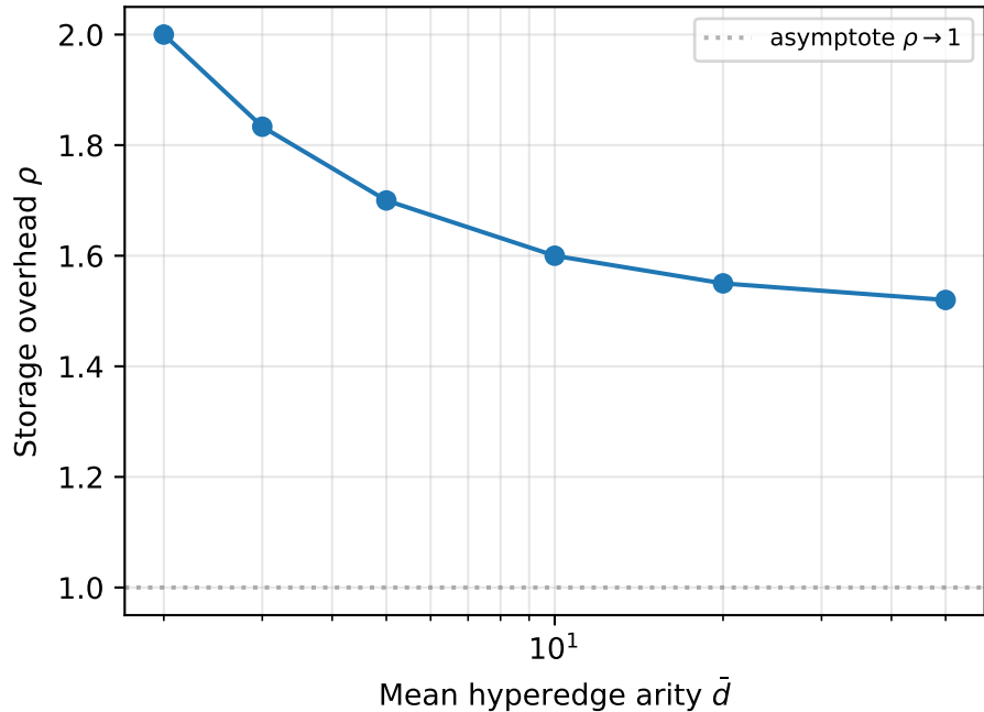
Prop. 4: \rho \rightarrow 1 for \bar{d} \gg \log n
