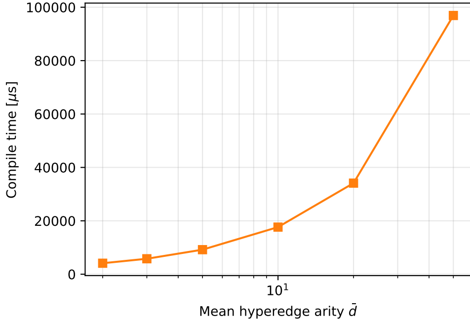
Compile time vs \bar{d} (highArity family, m = 200 )
