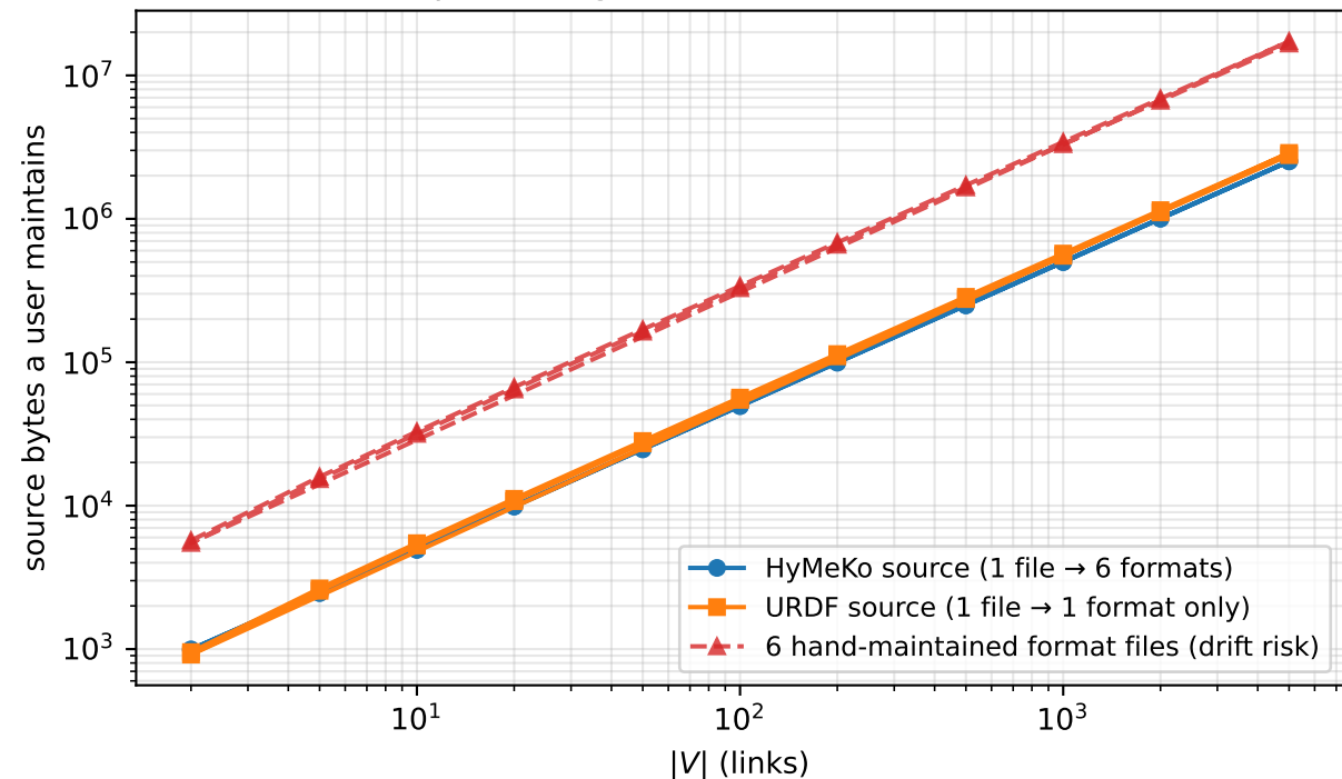
Description length to cover 6 coherent formats
