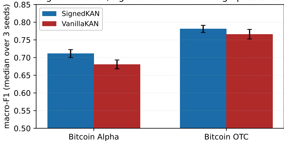
Sign-aware vs. sign-blind KAN on link sign prediction
