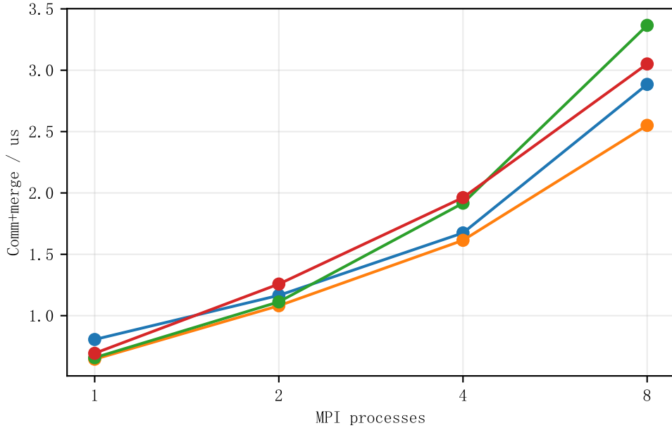
Kunpeng PBS: comm+merge
