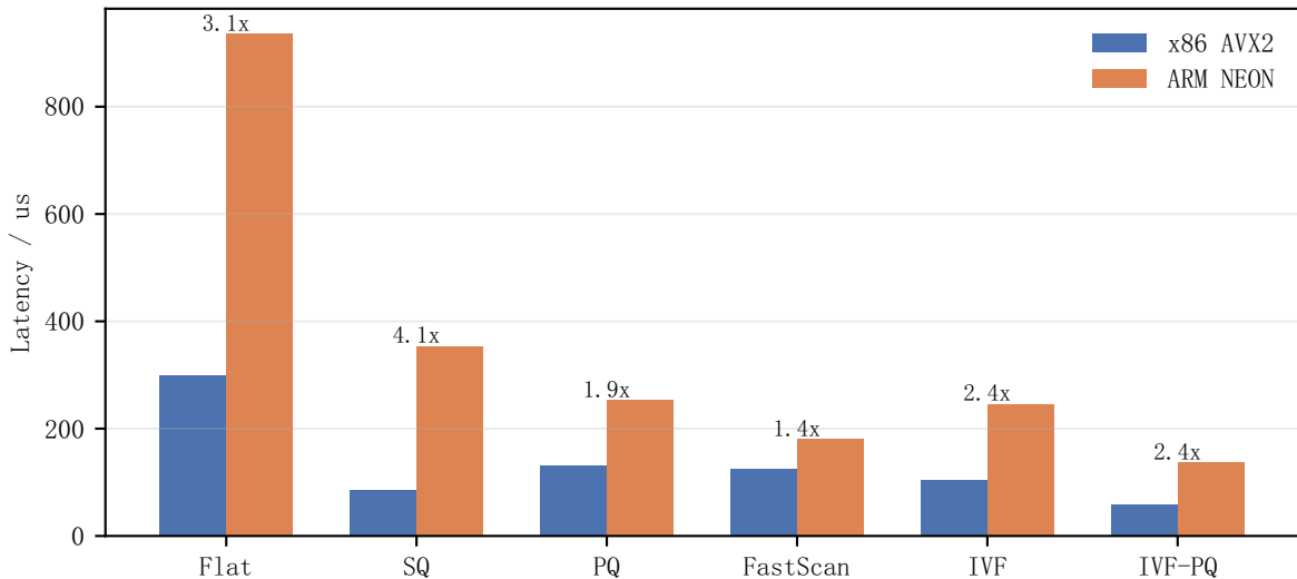
16-thread inter-query cross-platform latency
