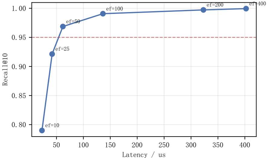
HNSW ef sweep (single thread)
