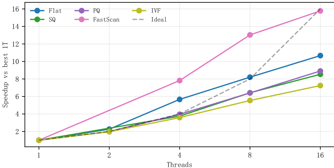
Inter-query scaling on i9-13900H
