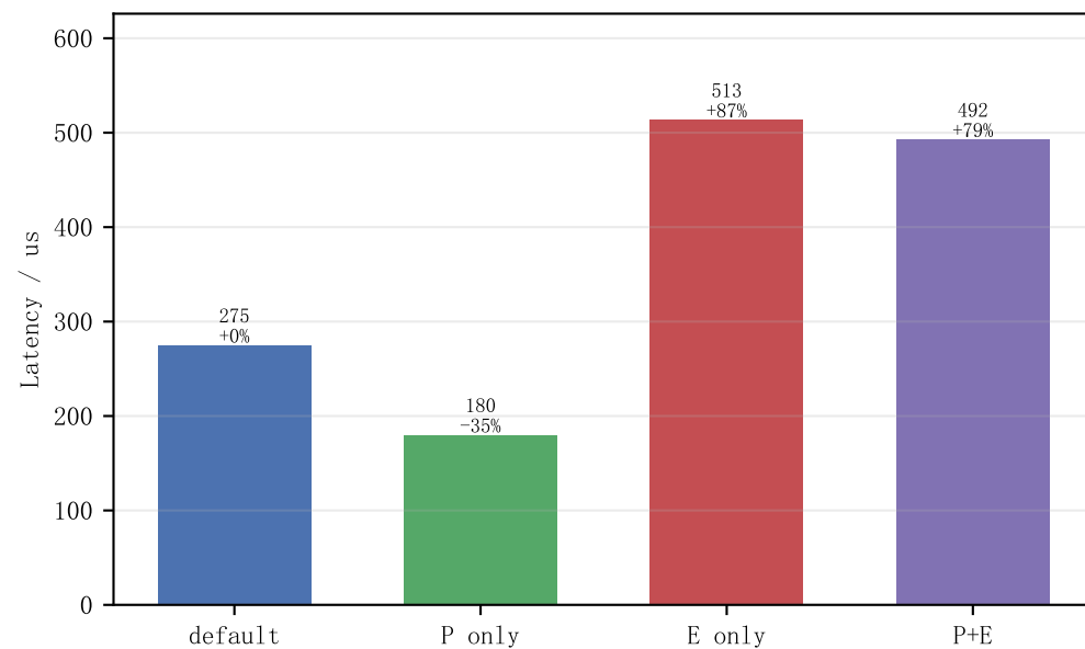
HNSW-on-HNSW
