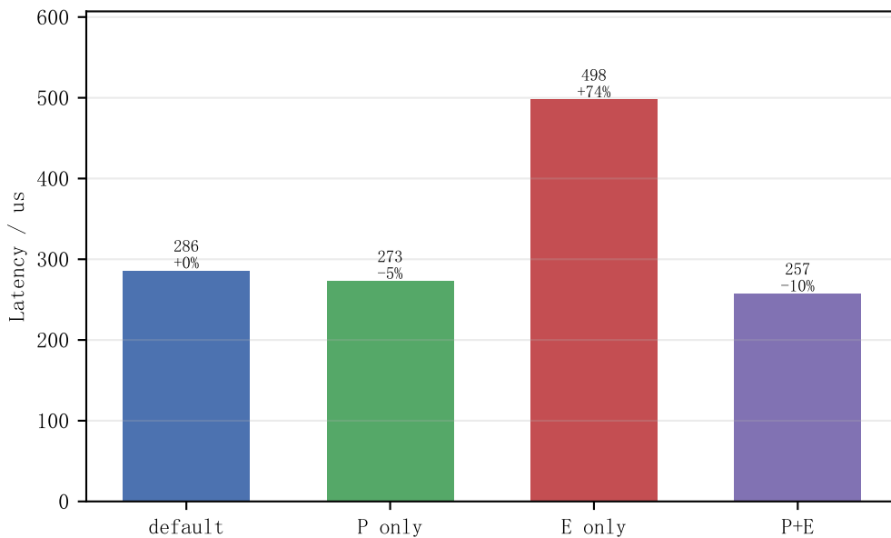
IVF+HNSW
