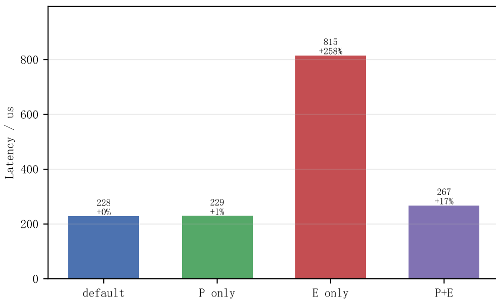
IVF+HNSW
