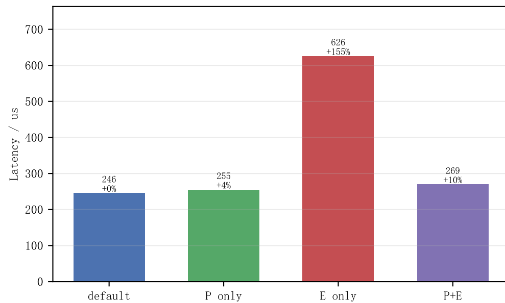
HNSW-on-HNSW
