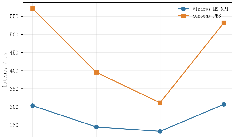
IVF+HNSW
