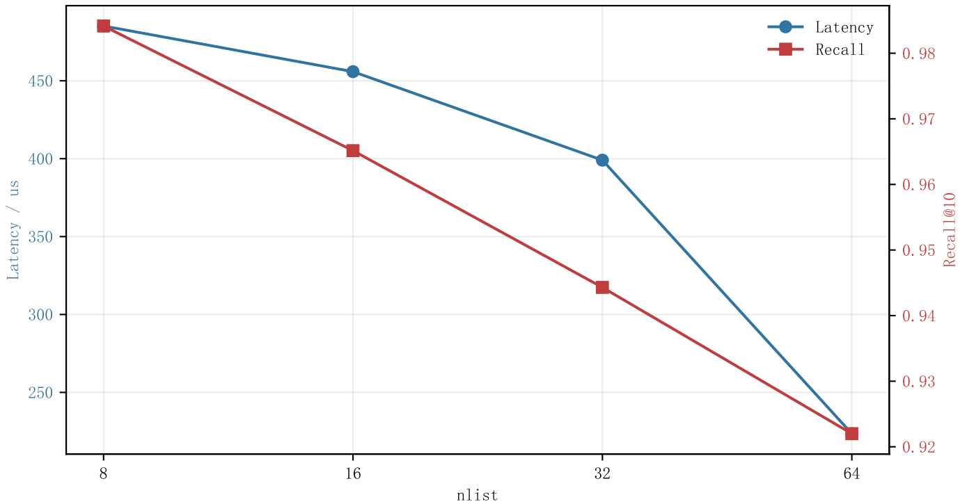
IVF-PQ nlist sweep at nprobe=4
