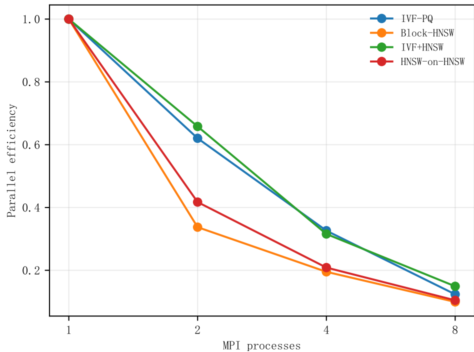
Windows MS-MPI strong scaling
