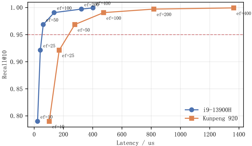
HNSW ef sweep (single thread)
