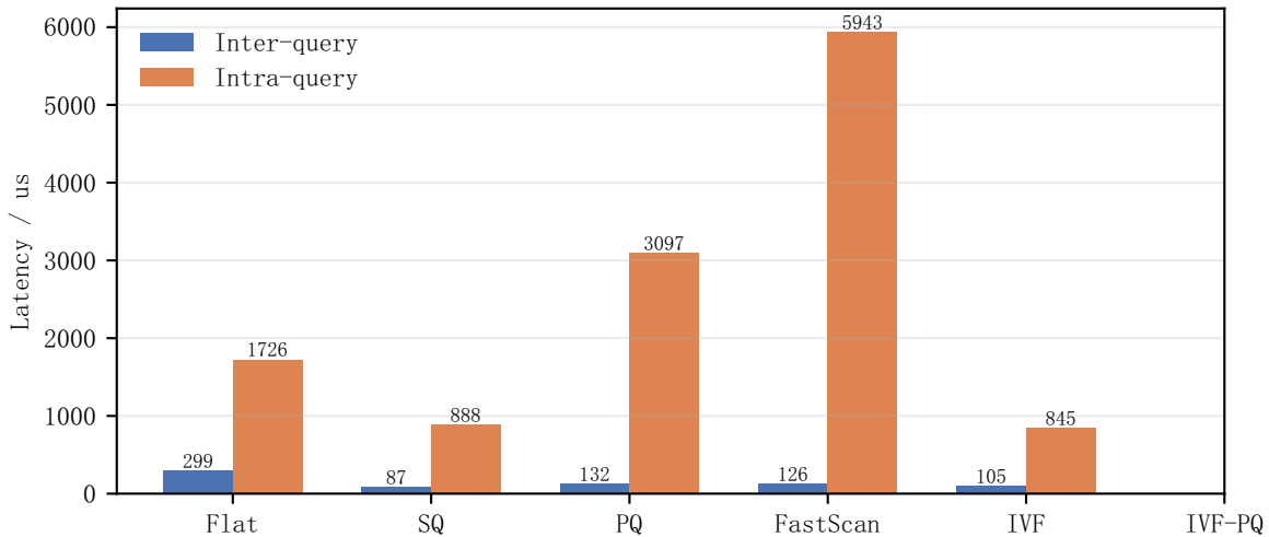
Best 16-thread inter-query vs intra-query latency
