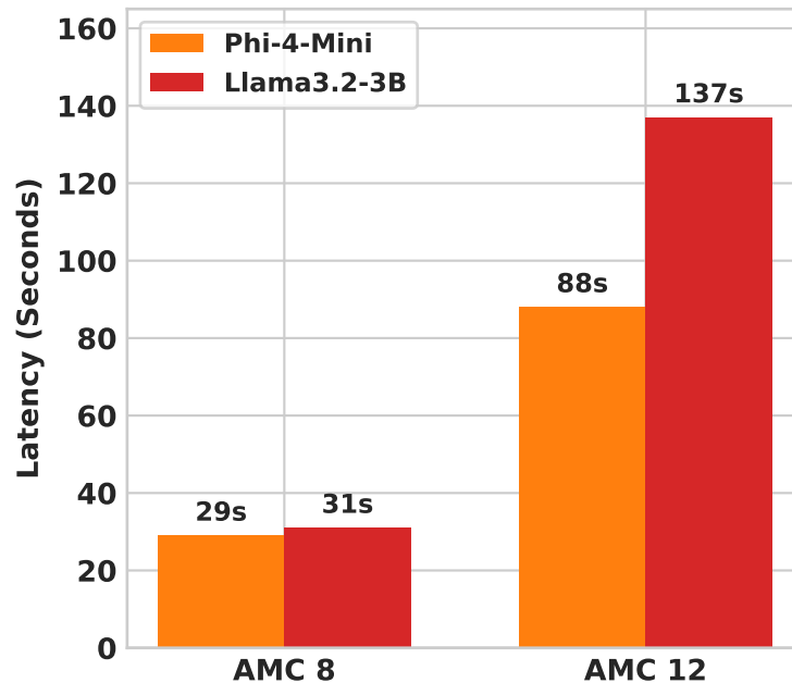
3.B) Latency Comparison
