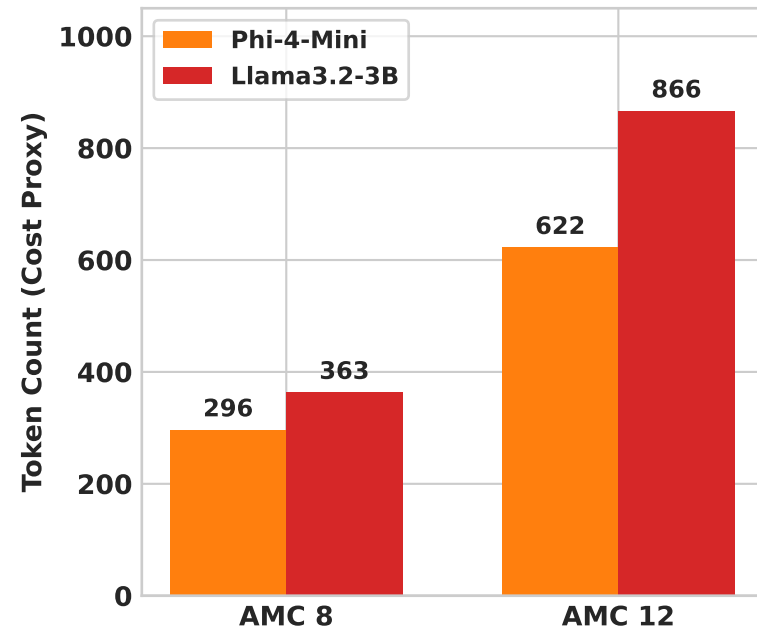
3.C) Computational Cost
