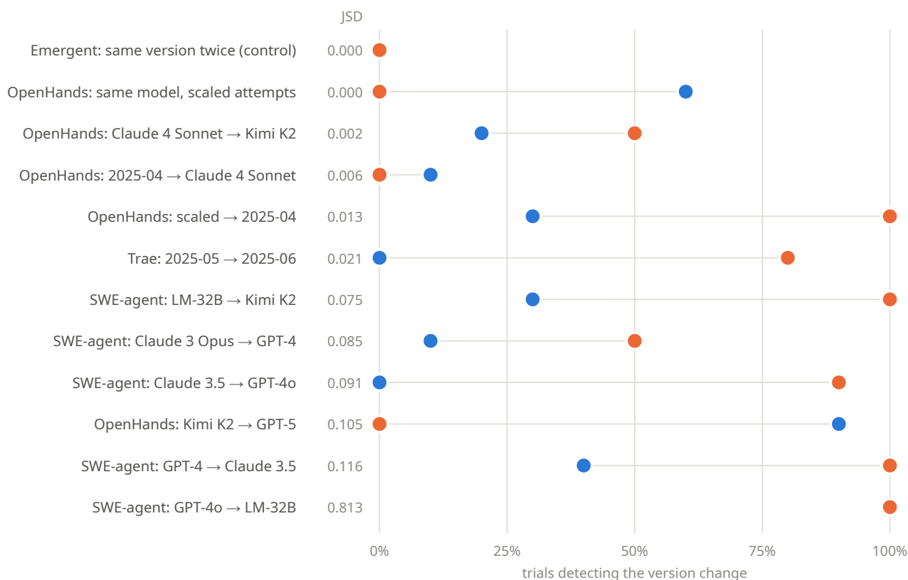
Figure 1. Version drift across 12 submission pairs. Each row is one pair; dots show the share of trials in which each channel alarmed. Rows are sorted by the Jensen–Shannon divergence (JSD) between the two submissions' overall tool distributions.
