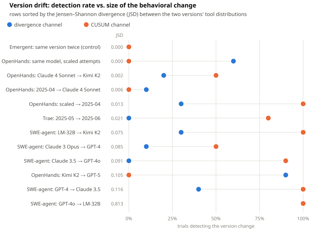
Figure 1. Version drift across 12 submission pairs. Each row is one pair; dots show the share of trials in which each channel alarmed. Rows are sorted by the Jensen–Shannon divergence (JSD) between
