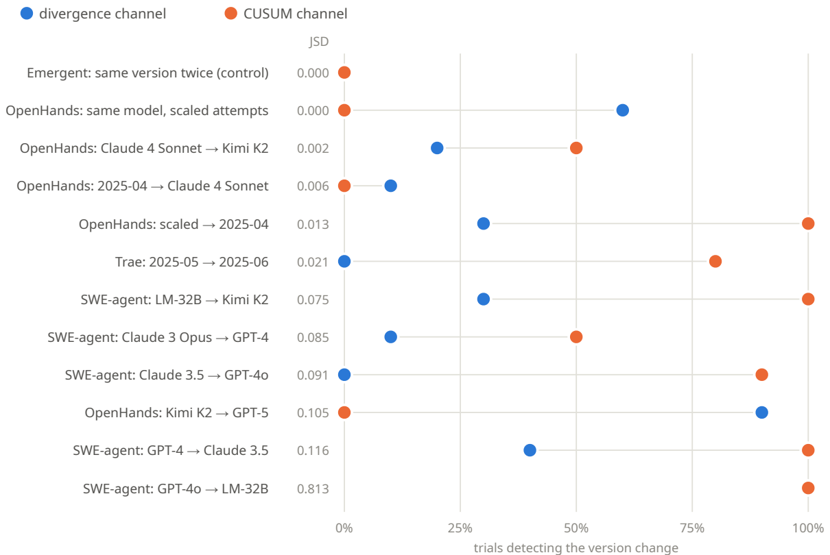
Figure 1. Version drift across 12 submission pairs. Each row is one pair; dots show the share of trials in which each channel alarmed. Rows are sorted by the Jensen–Shannon divergence (JSD) between the two submissions' overall tool distributions.
