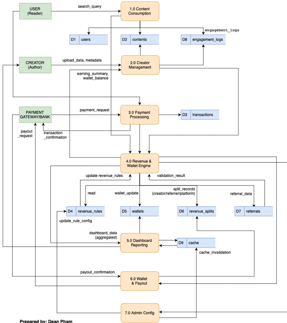
Fig 1.2: DFD Level 1 - Fintech Monetization Platform
