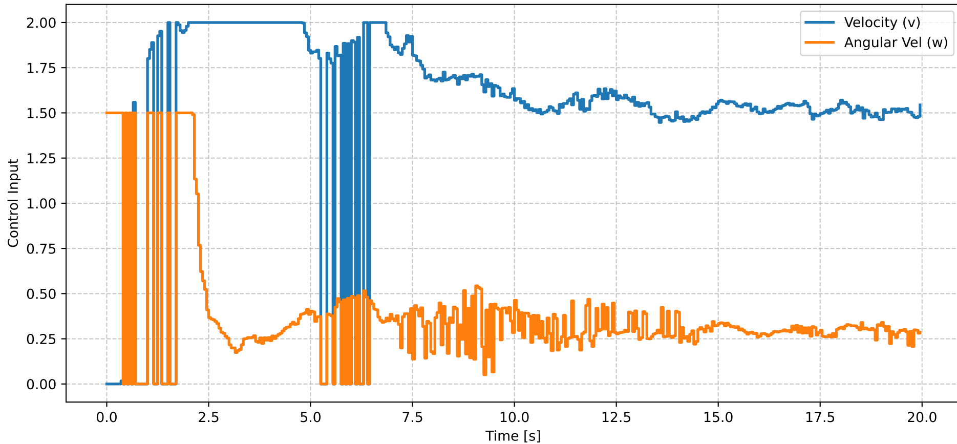
Figure 2: Control Inputs
