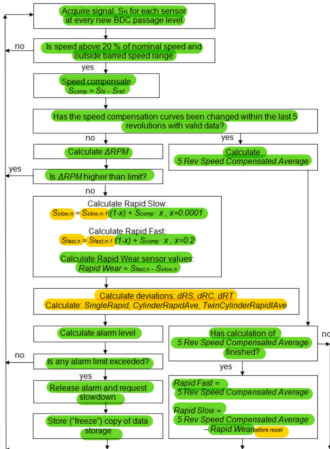
Figure 4.3, Flow chart for rapid wear evaluation.
