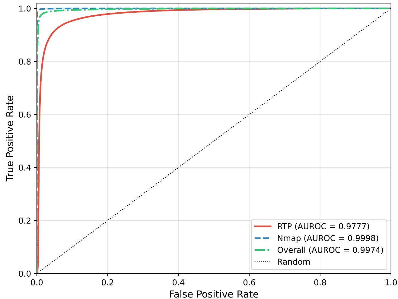
ROC Curve
