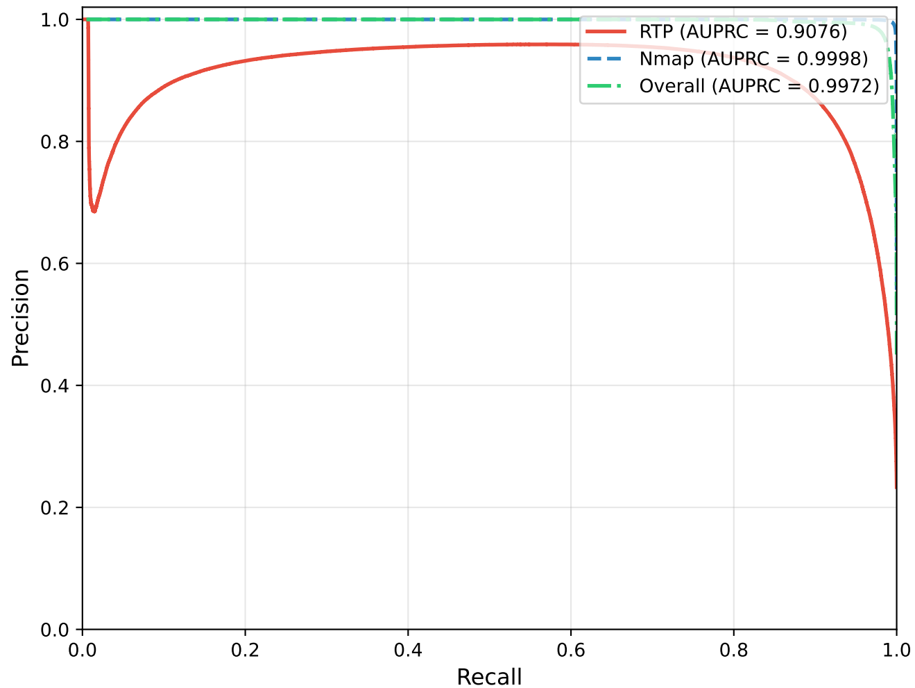
Precision-Recall Curve
