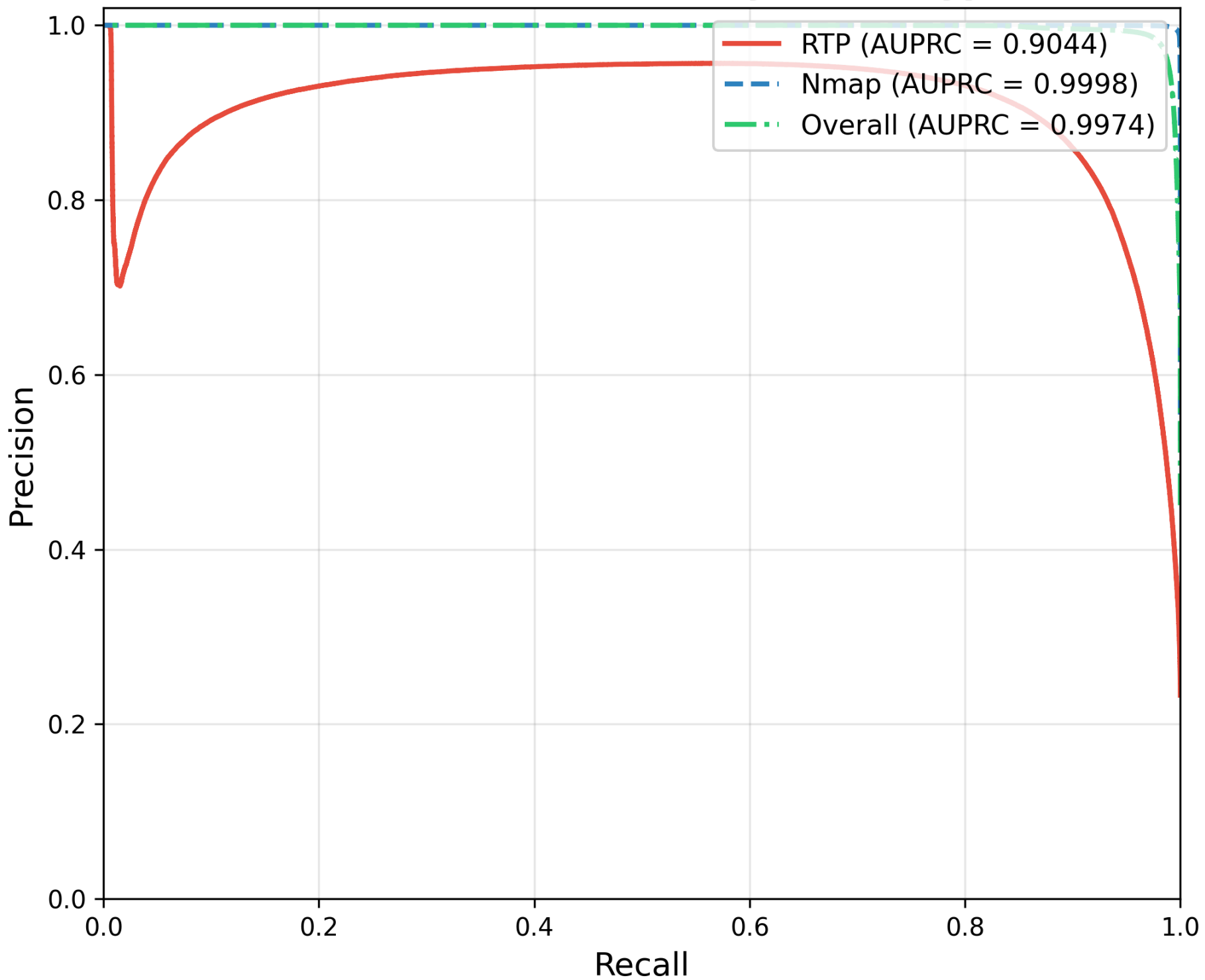
Precision-Recall Curve by Attack Type
