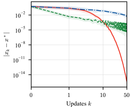
Current iterate
