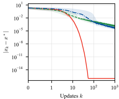
Current iterate
