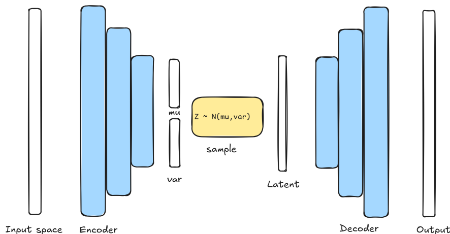
Figure 2: variational autoencoder. Notice that this sampling procedure complicates backpropagation. To alleviate this, we use reparameterization trick.
