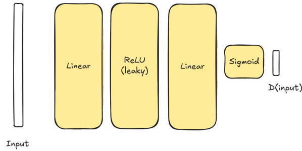
Figure 4: GAN discriminator diagram.
