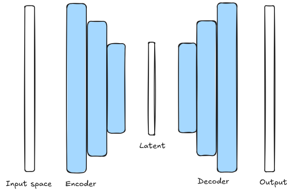
Figure 1: traditional autoencoder. Typically is optimized using a reconstruction objective between input and output.
