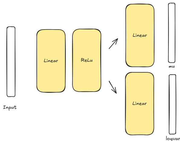
Figure 3: VAE encoder diagram.
