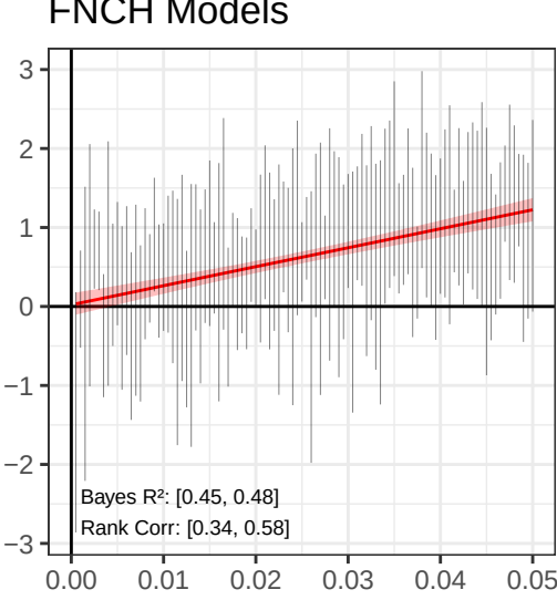
FNCH Models
