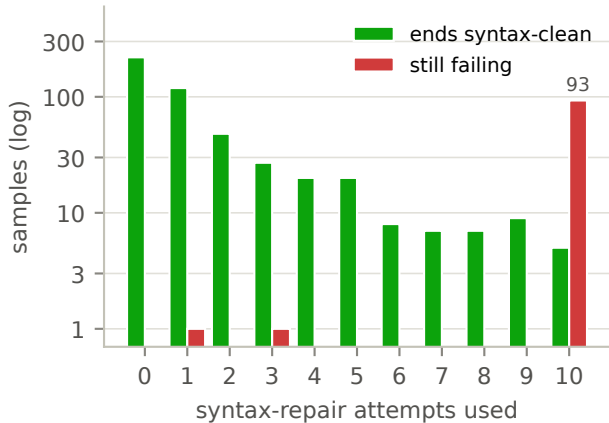
Syntax repair
