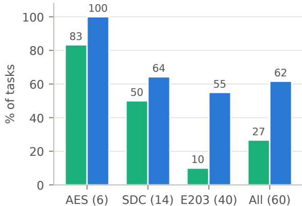
Syntax rate (%)
