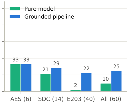
Pass rate (%)
