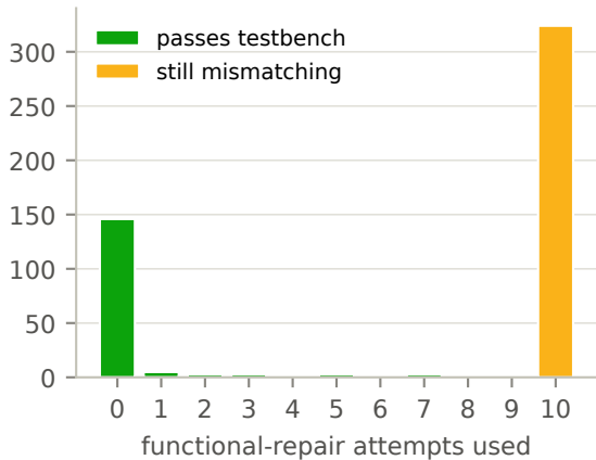
Functional repair (compiling samples)
