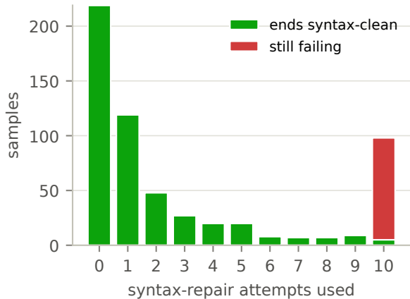
Syntax repair
