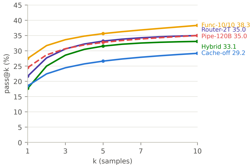
Figure 6.3: Unbiased pass@k for k = 1-10 across five arms on one axis. Normalizing at k \leq 10 lets every 60 \times 10 run be read together with the 60 \times 20 runs (whose curves the estimator subsamples). System design separates the curves more than model scale does.
