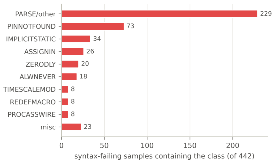
Figure 6.9: Verilator diagnostic classes among the 442 syntax-failing samples of CACHE-OFF (a sample can carry several classes).
